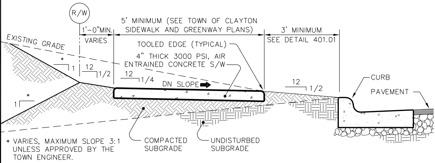
TYPICAL SIDEWALK with UTILITY STRIP
