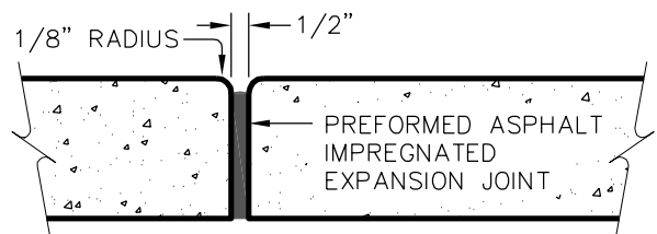
TYPICAL EXPANSION JOINT DETAIL
